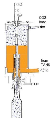
CO2 INJECTION for Compensation
