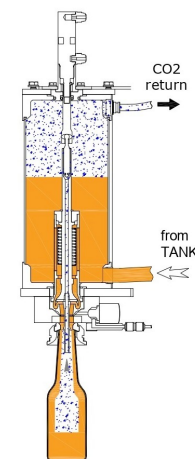
VALVE OPENED for FILLING
